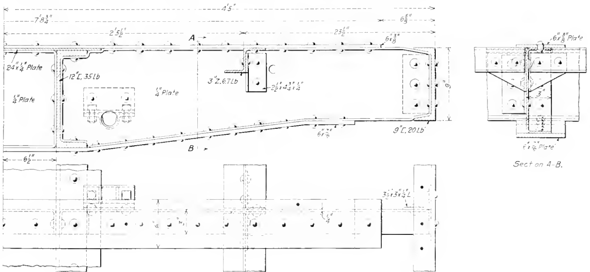
Details of Main Cross-tie - Santa Fe Stock Car
